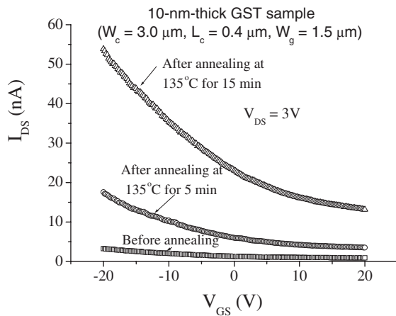
Fig. 7. Current control effect of 10-nm-thick GST device before annealing (amorphous) and after annealing at 5 and 15 min (crystalline).
